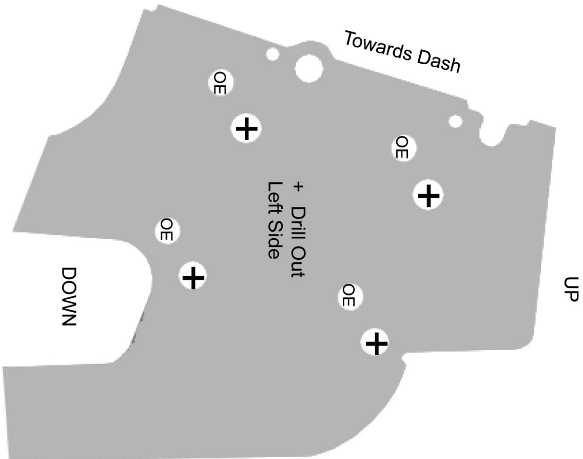
AVNC mounting template for LAND CRUISER 100 SERIES (IFS)
